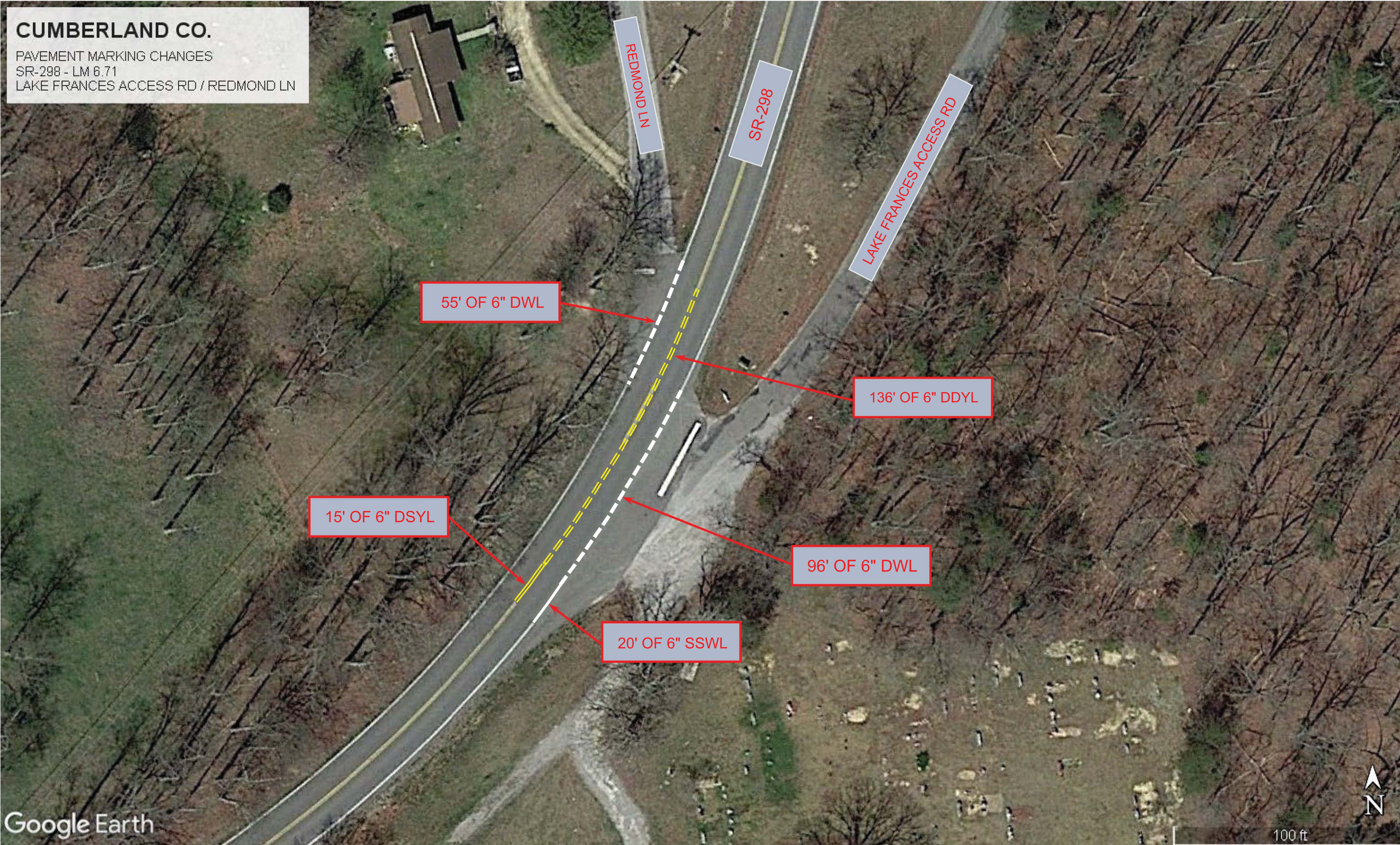
DETAIL OF PAVEMENT MARKING CHANGES AT LAKE FRANCES ACCESS RD / REDMOND LN SR-298 @ LM 6.71
